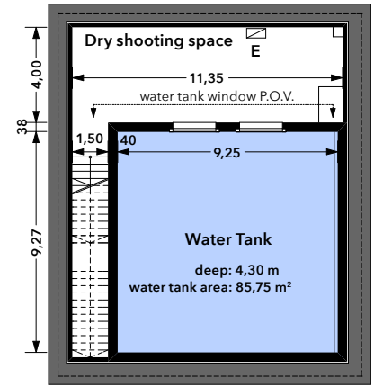
BASEMENT PLAN
